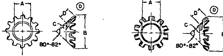
ACCEPTABLE DESIGNS
